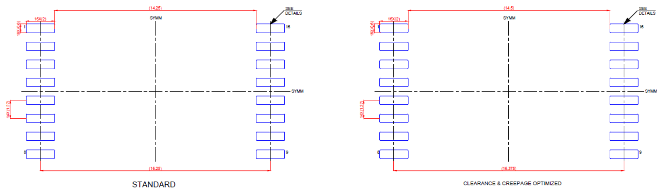
LAND PATTERN EXAMPLE(mm)
