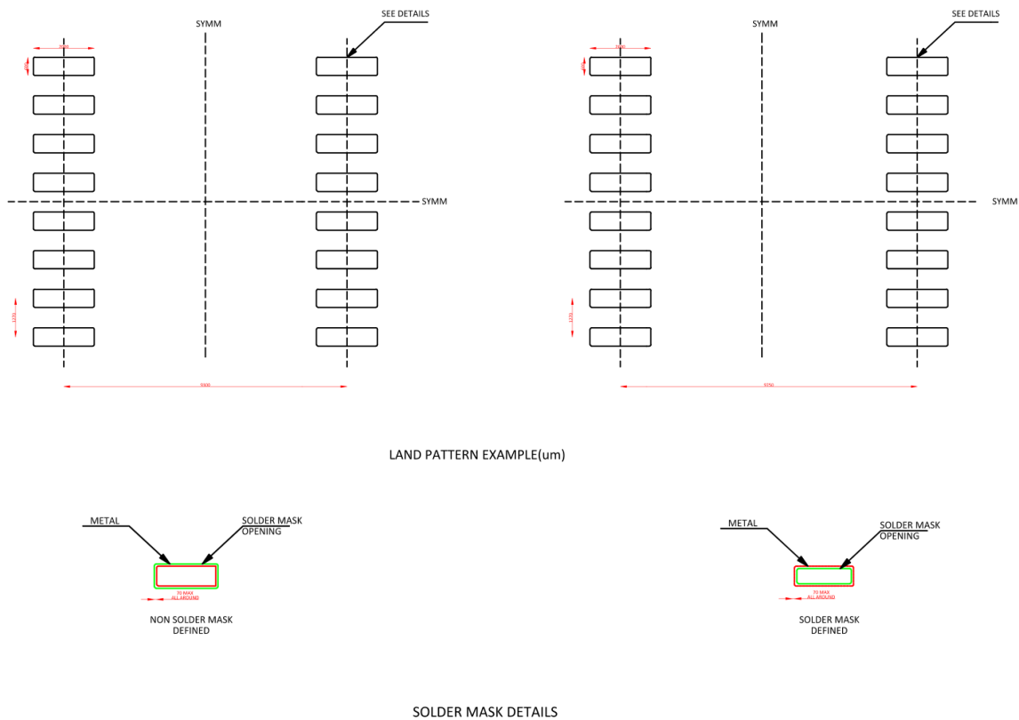
Figure 9.2 SOP16(300mil) Package Board Layout Example
