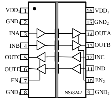
Figure 1.3 NSi8242W Package
