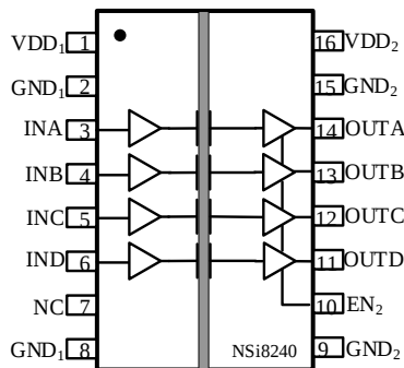
Figure 1.1 NSi8240W Package
