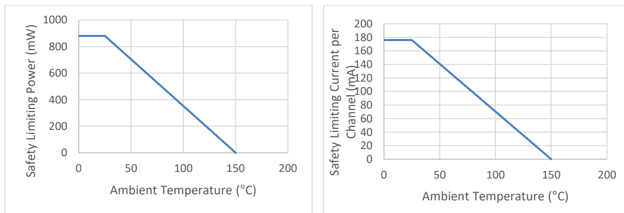
Figure 6.2 NSi824xS Thermal derating Curve, Dependence of Safety Limiting Values with Case Temperature per DIN VDE V 0884-11
