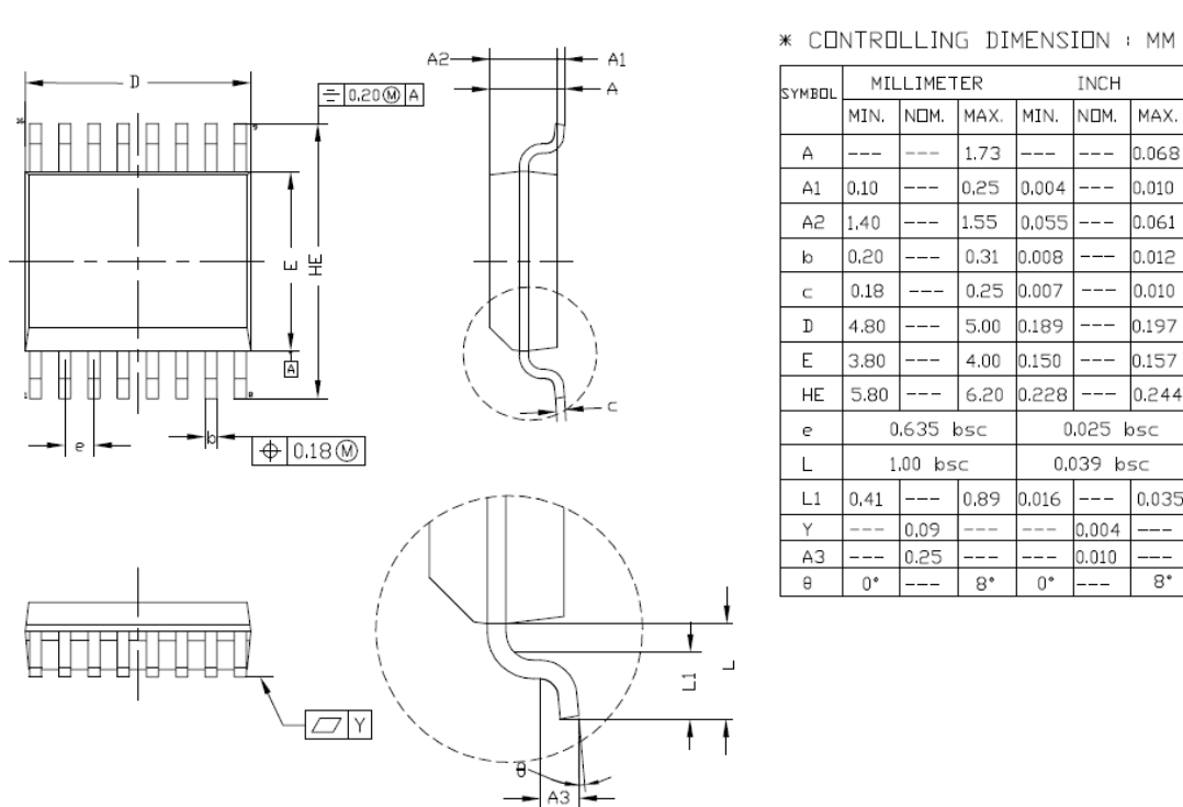
Figure 9.5 SSOP16 Package Shape and Dimension in millimeters
